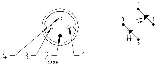
Pinout F
