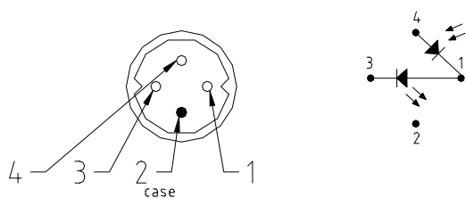
Pinout Q
