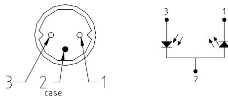
Pinout C
