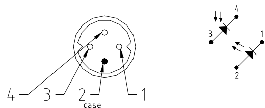
Pinout E
