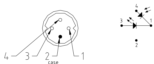
Pinout O
