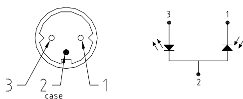
Pinout M
