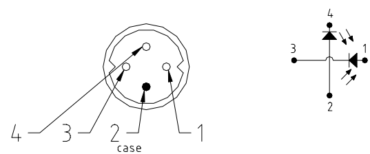
Pinout H
