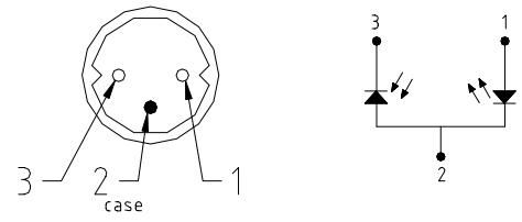
Pinout B
